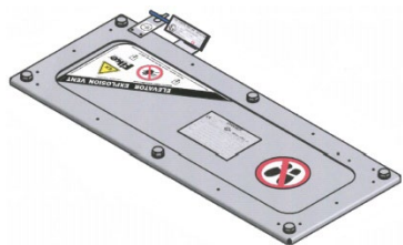
EleGuard Vent with Rupture Indicator
