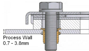
EleGuard Process Attachment
